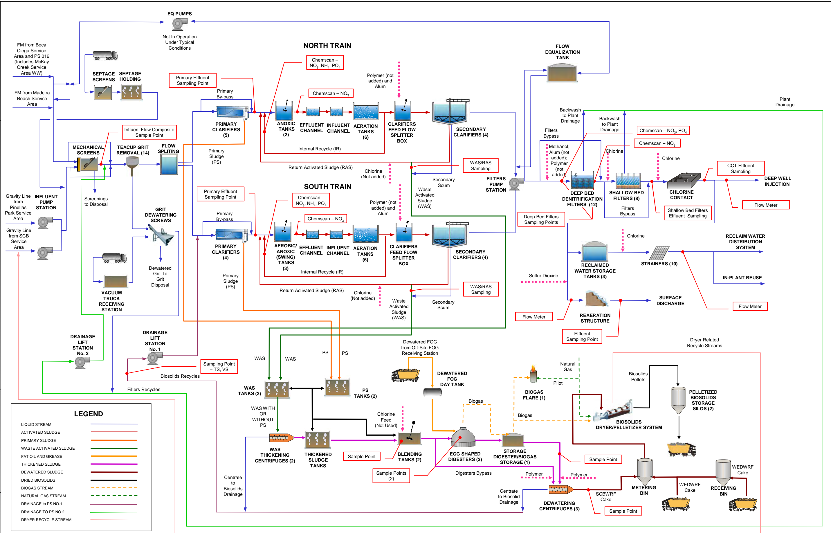
SCBWRF Process Diagram
