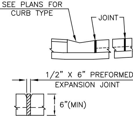
JOINT DETAIL
