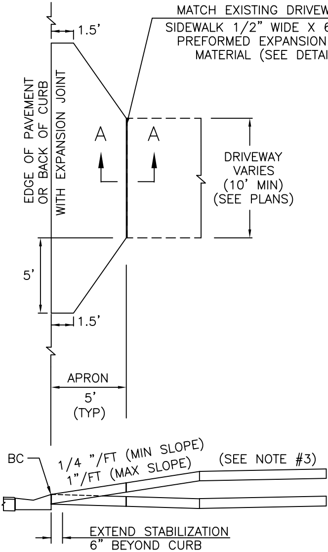
PLAN AND PROFILE VIEW
