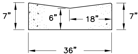
VALLEY GUTTER SECTION A-A
