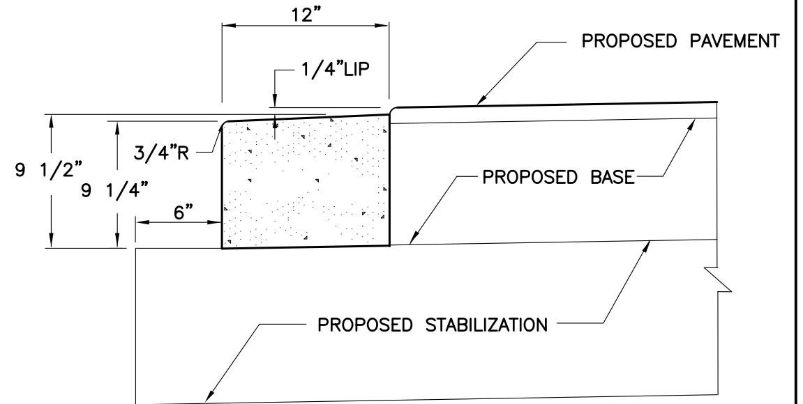
PROFILE VIEW OF HEADER CURB
