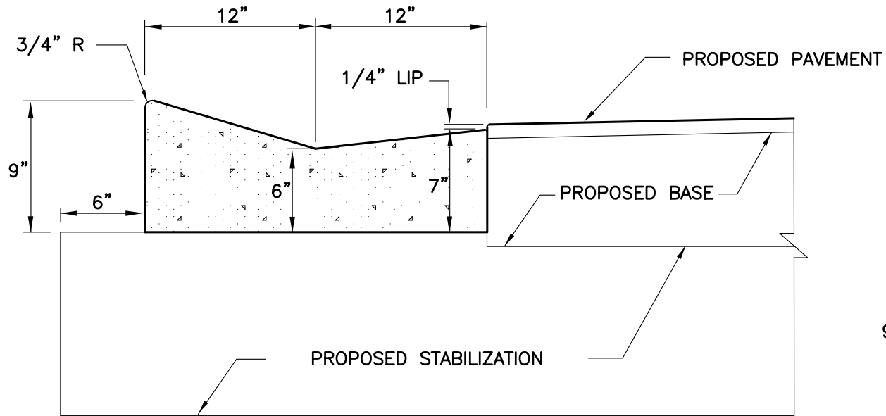
PROFILE VIEW OF CURB & GUTTER
