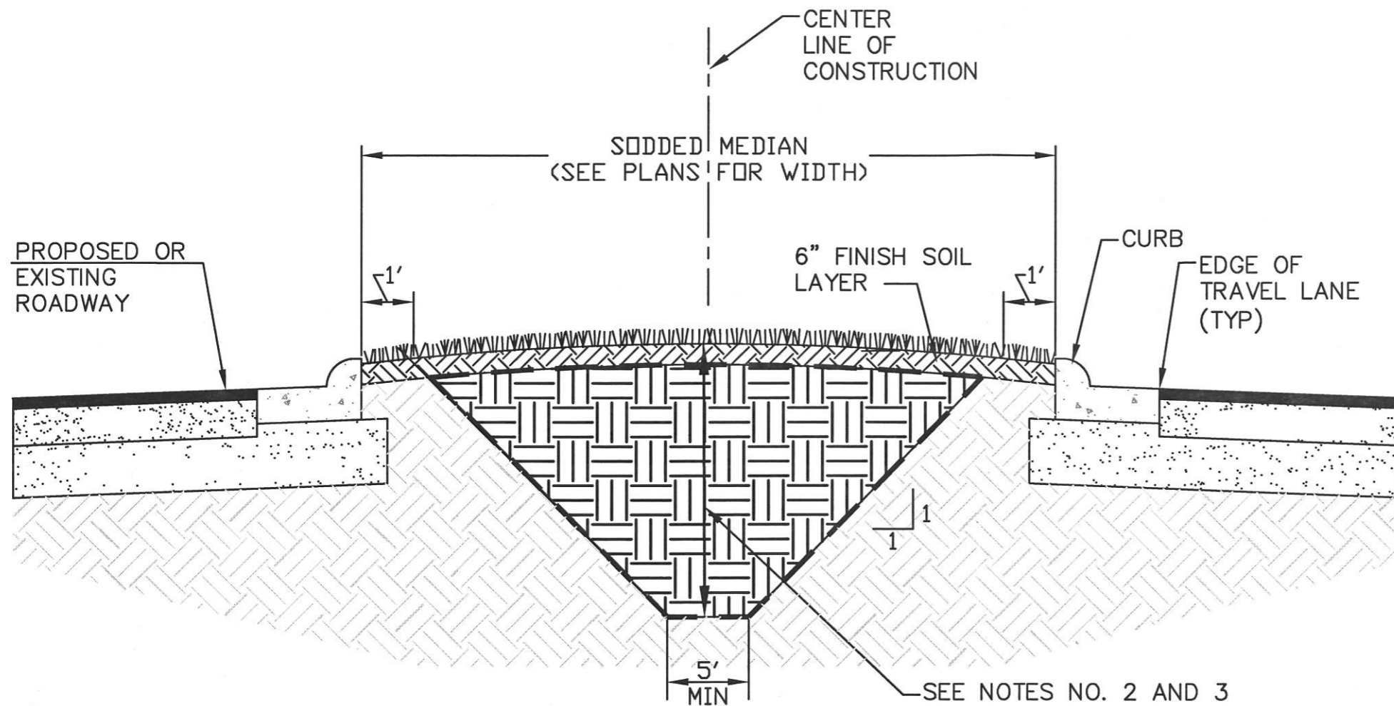
TYPICAL SECTION
